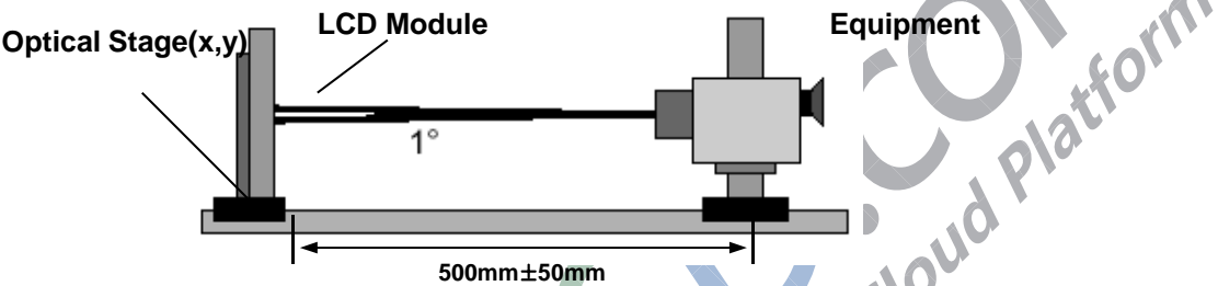
FIG. 1 Optical Characteristic Measurement Equipment and Method
