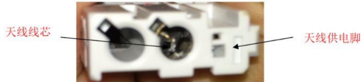
PORT F
